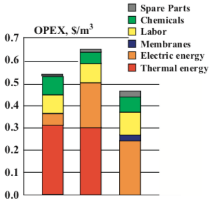
Fig. 44. OPEX for conventional desalination technologies(GWI 2010) [6].
