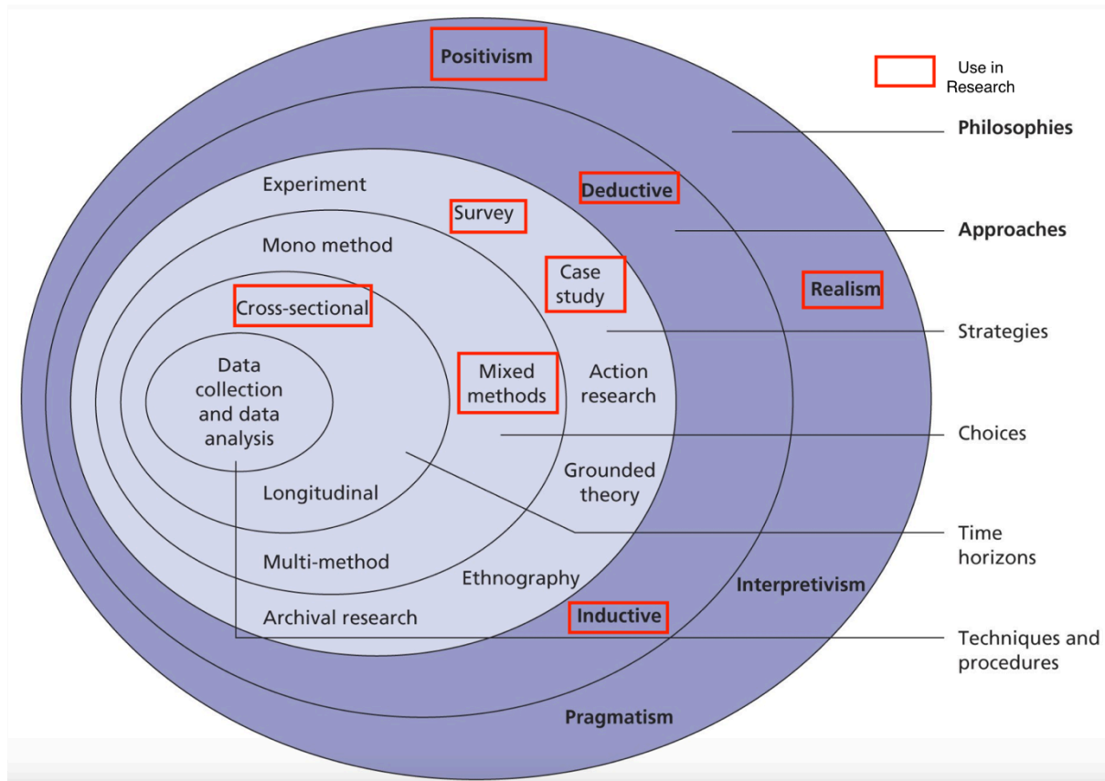
Figure 1: Research Onion
